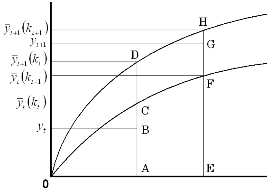
Figure A2. Illustration of Tripartite Decomposition
