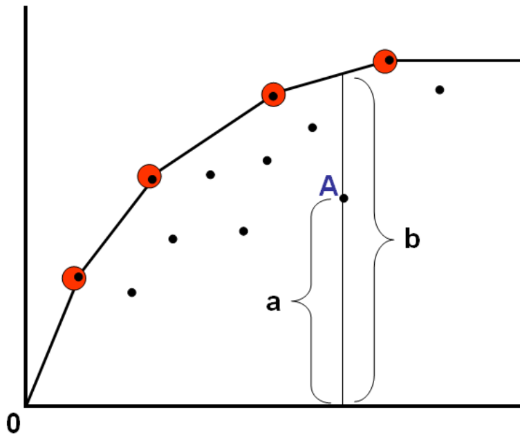
Figure A1: The concept of Data Envelopment Analysis
